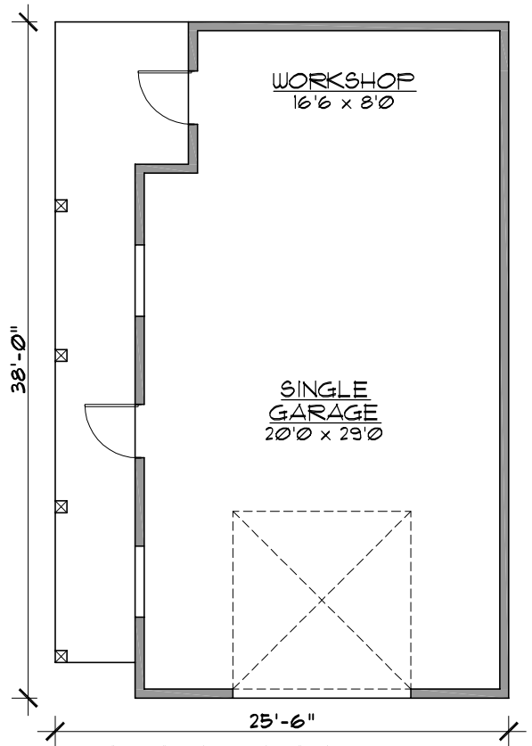
GARAGE PLAN
